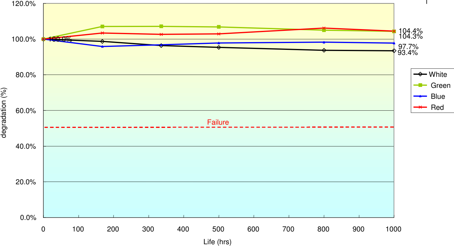
Room Temp. Operation Life
